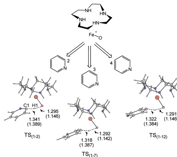
Figure 5. The attack position of the \text{FeO}^+ toward the C atom on the pyridine ring and the optimized structures of the C–H activation TSs along different paths. (Bond lengths of the optimized structures on the quartet are presented, and the ones on the sextet are listed in parentheses, bond lengths in Å.)
