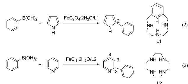
Scheme 2. Iron–MCPA Complex Catalyzed Direct Suzuki–Miyaura Reaction
