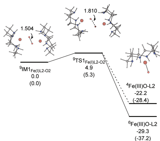
Figure 4. PCM energies (in kcal/mol) in acetic acid for the optimized structures involved in the recovery process. PCM energies (in kcal/mol) in pyridine are listed in parentheses. (The solid curve represents the sextet surface, and the dashed one represents the quartet surface.)
